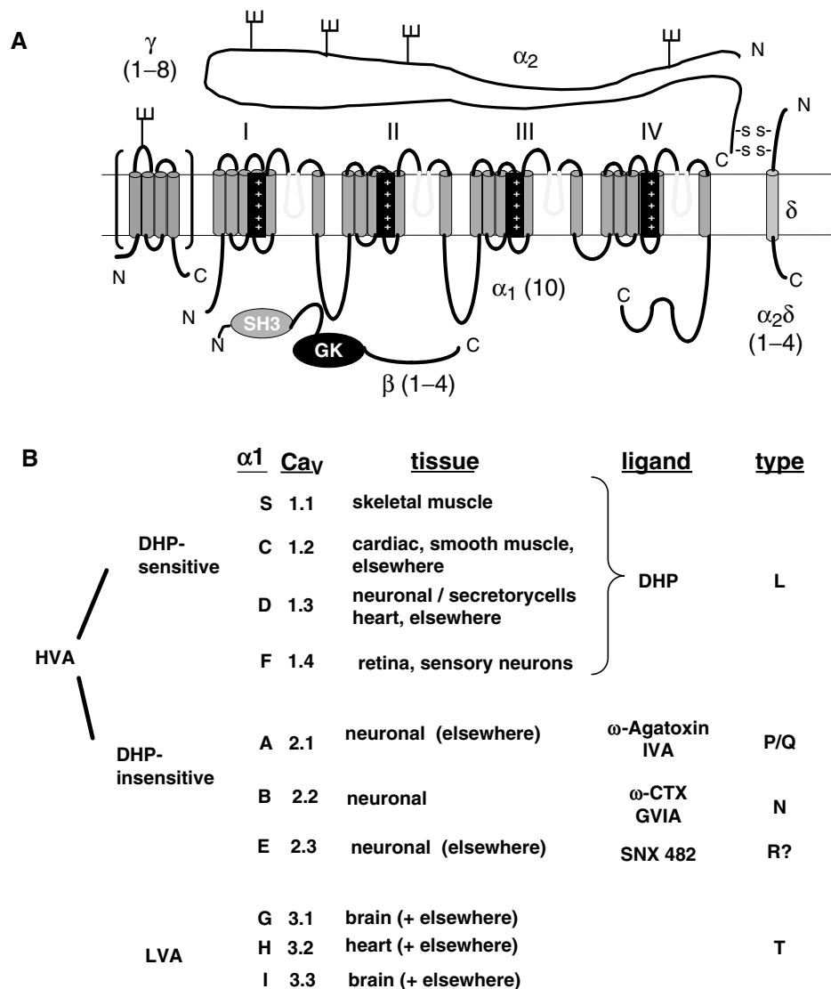
FIGURE 20.3 Voltage-gated calcium channels, like sodium channels, comprise a single functional \alpha -subunit, but the accessory subunits ( \alpha , \beta , \gamma , \delta , \alpha_2\delta ) associated with these channels are more complex. Channels are divided into HVA (high voltage activated) or LVA (low voltage activated) and DHP (dihydropyridine) sensitive or insensitive. The \alpha -subunits are now classified using a numerical designation.
