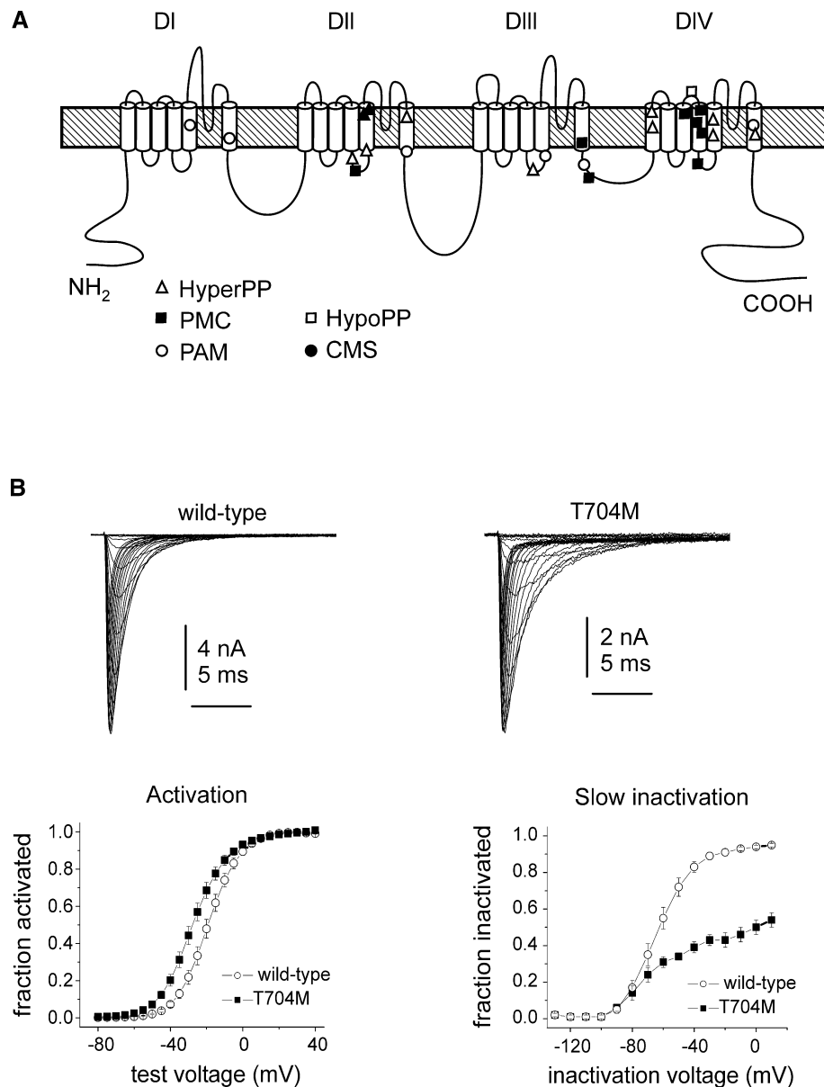
FIGURE 18.5 Mutations in Na v 1.4 are associated with several muscle disorders. A: Schematic representation of the voltage-gated sodium channel \alpha -subunit. Locations of mutations associated with HyperPP, PMC, PAM, HypoPP, and CMS are shown. B: The HyperPP T704M mutation alters the voltage dependence of activation ( bottom left ) and impairs slow inactivation ( bottom right ) of Na v 1.4 sodium currents.
