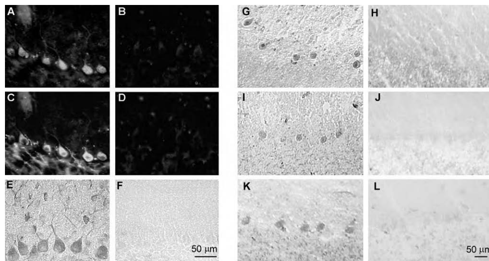
FIGURE 19.10 Annexin, which facilitates insertion of functional \text{Na}_v1.8 channels into the cell membrane, is up-regulated and co-expressed with \text{Na}_v1.8 in Purkinje cells in EAE and MS. Left Panel : \text{Na}_v1.8 ( A ) and annexinII/p11 ( B ) are up-regulated in Purkinje neurons in EAE vs control ( B and D , respectively). AnnexinII/p11 immunostaining extends along the proximal portion of the dendritic tree in EAE ( E ) but not in control ( F ). Right Panels : Up-regulation of \text{Na}_v1.8 and annexinII/p11 in human MS tissue. \text{Na}_v1.8 is up-regulated in human MS Purkinje neurons ( G ) vs control ( H ). Up-regulated expression of annexinII/p11 is shown for two MS cases ( I and K ) in comparison to controls ( J and L ). Modified from Craner MJ et al. (2003b).
