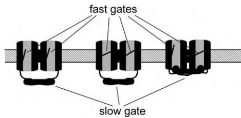
FIGURE 18.4 Schematic representation of the double-barreled structure of CIC-1 chloride channels. Fast gates act independently to control the activity of two distinct ionic pathways. A common slow gate controls the activity of the two ionic pathways simultaneously. GMC mutations can alter either fast or slow gating.
