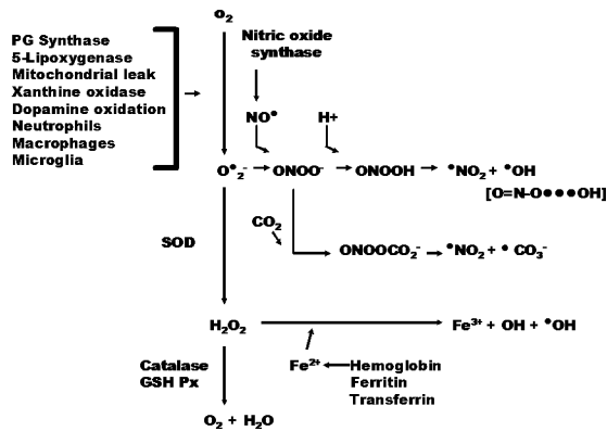
FIGURE 3.2 Biochemistry of reactive oxygen species generation and free radical formation in the injured CNS. PG synthase = prostaglandin synthase; O_2^- = superoxide radical; NO^+ = nitric oxide; ONO_2^- = peroxynitrite anion; ONOOH = peroxynitrous acid; NO_2^- = nitrogen dioxide radical; OH = hydroxyl radical; ONOOCO_2^- = nitrosoperoxocarbonate; CO_3^- = carbonate radical; SOD = superoxide dismutase; Fe^{2+} = ferrous iron; Fe^{3+} = ferric iron; GSH Px = glutathione peroxidase.
