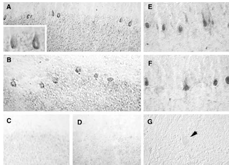
FIGURE 19.9 Expression of the Sensory Neuron Specific (SNS) sodium channel \text{Na}_v1.8 is up-regulated in cerebellar Purkinje neurons in patients with MS. In situ hybridization with \text{Na}_v1.8 specific antisense riboprobes demonstrates increased \text{Na}_v1.8 mRNA in Purkinje cells from MS patients obtained at postmortem ( A, B ), compared to controls without neurological disease ( C ). No signal is present following hybridization with sense riboprobe ( D ). Immunocytochemistry with SNS-specific antibodies demonstrates up-regulation of \text{Na}_v1.8 channel protein in Purkinje cells from MS patients ( E, F ) compared to controls ( G ; arrowhead indicates Purkinje cell). A : x 120, inset x 280; B–D : x 165; E–G : x 175. From Black JA et al. (2000).
